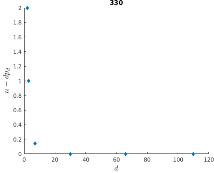
Figure 4: Decrease of n - dp_d for n = 330 .
